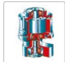
Composite impellers and rotor Lubrication-free, works without oil. Counterweight system to guarantee smooth operation.
