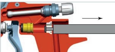
Disassembly Fig.13.1
